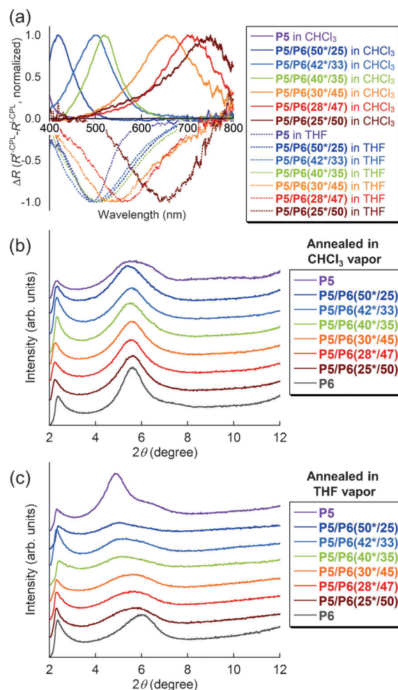
Figure 2. a) Difference reflection spectra of P5 and P5/P6 (x*/y) annealed in \text{CHCl}_3 (solid lines) or THF vapor (dotted lines). P6 did not exhibit selective reflection. b, c) XRD ( \text{Cu K}\alpha ) patterns of polymer films annealed in \text{CHCl}_3 (b) or THF vapor (c).
